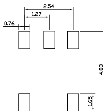
Recommended PAD Layout
