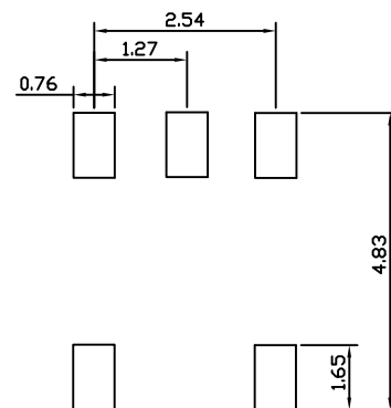
Recommended PAD Layout Top View
