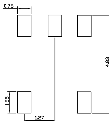
Recommend PAD layout
