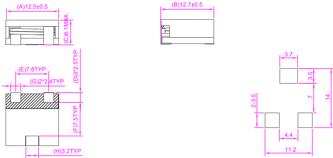
SUGGESTED PAD LAYOUT
