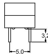
Unless otherwise specified all tolerances are:±0.25 in mm
