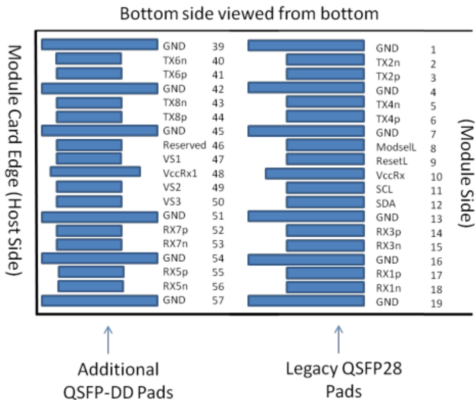
Figure1 QSFP-DD Pin Assignment
