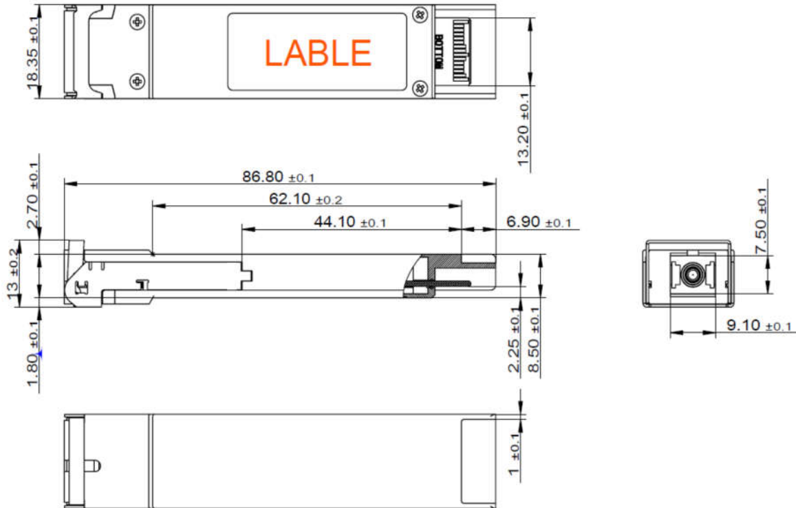
Figure 8 Package Outline
